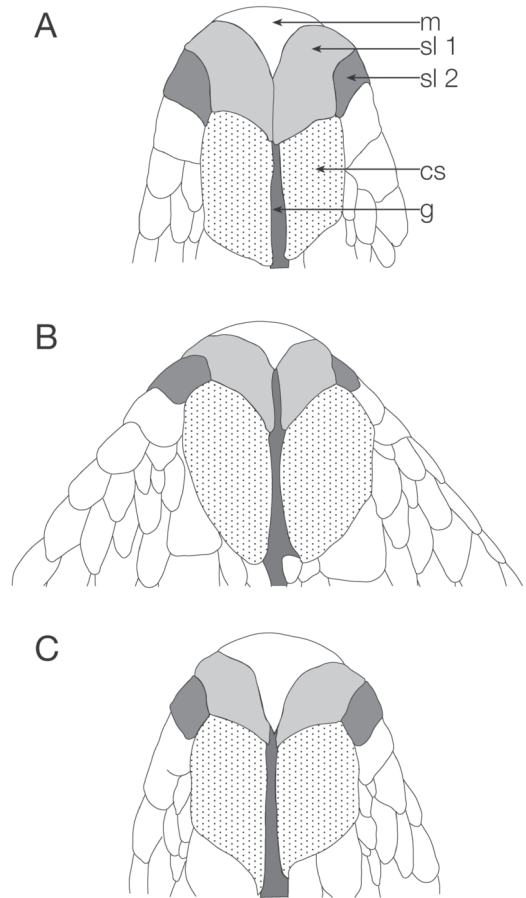
FIG. 2. -- Ventral aspect of head of (A) Crotalus stejnegeri , UTA R-6234; (B) C. lannomi , BYU 23,800; and (C) C. ericsmithi , UTA R-55372, showing differences in scalation. Shape of lower jaw of C. lannomi somewhat distorted during preservation. Abbreviations as follows: m, mental; sl 1, first supralabial; sl 2, second supralabial; cs, chinshield; g, midventral gular fold.
