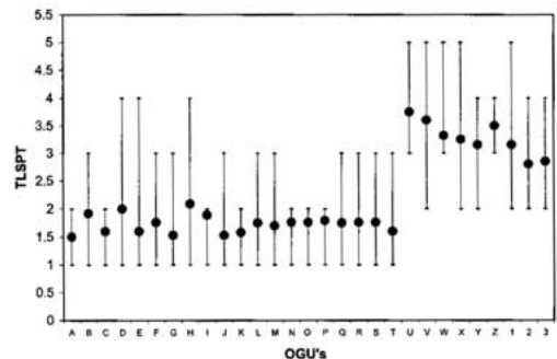
FIG. 4. Analysis of population mean for TLSPT. Range of values for each OGU is indicated.
