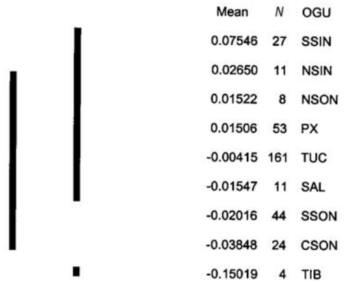
FIG. 7. Tukey's studentized range (HSD) test, for the third principal component for the western group.
