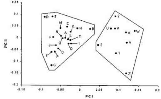
FIG. 6. Results of the PCA. Letters and numbers represent the Geographic Units and correspond to those listed in Table 1.
