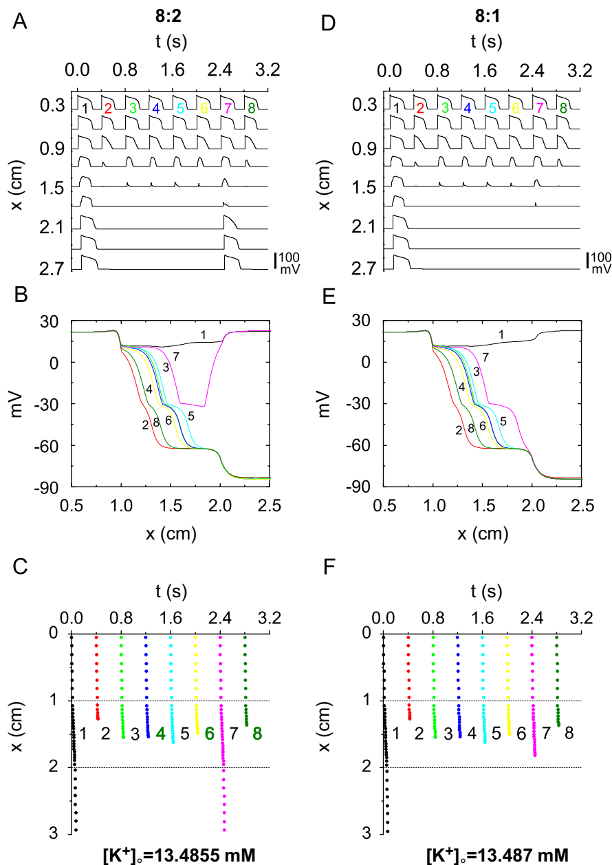
Fig. 5. Period-8 rhythms : Left column (A–C): 8:2 rhythm, [K^+]_o = 13.4855 \text{ mM} ; right column (D–F): 8:1 rhythm, [K^+]_o = 13.487 \text{ mM} . Same format as Fig. 2.
