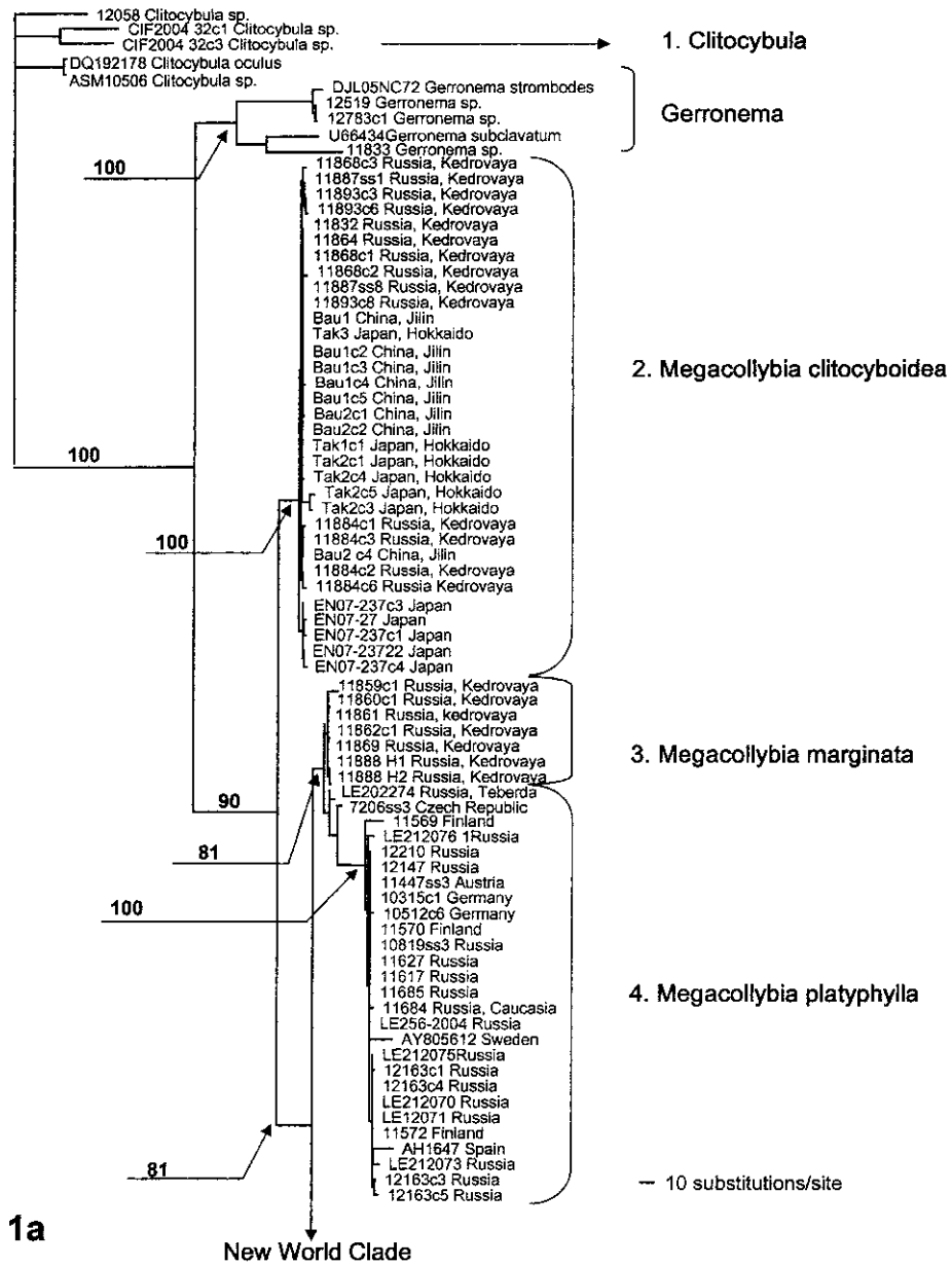
FIG 1a, b. One of 1000 most parsimonious trees of length 1230 steps. Boot strap support is given to the left of the node, followed by the Bayesian posterior probability. Of 914 total characters: All characters were unordered and of equal weight; 322 characters were constant, 93 variable characters were parsimony-uninformative, 499 characters were parsimony-informative. Gaps were treated as “fifth base.” Numbers adjacent to clades refer to numbers in manuscript under “results.”
