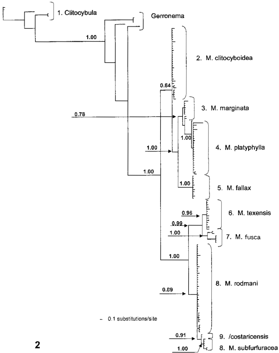
FIG. 2. Bayesian analysis using a GST+G model. Posterior probabilities are given to the left of the node.
